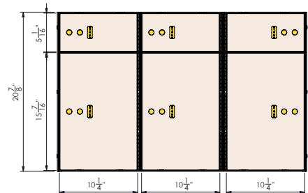
SS-7PV3 3 - 5 x 10 Stainless Steel Doors 3 - 15 x 10 Stainless
