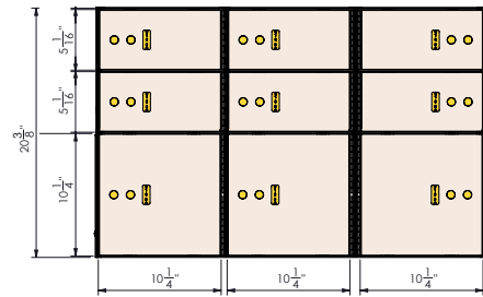
SS-5PV3 6 - 5 x 10 Stainless Steel Doors 3 - 10 x 10 Stainless Steel Doors
