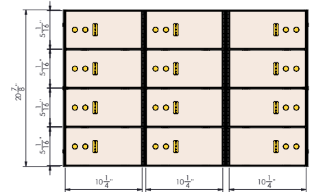
SS-4PV3 12 - 5 x 10 Stainless Steel Doors
