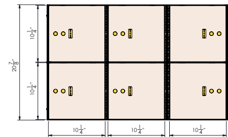
SS-6PV3 6 - 10 x 10 Stainless Steel Doors
