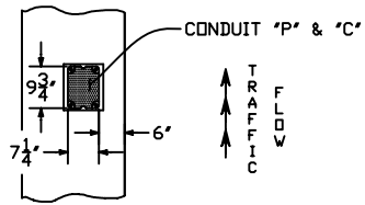
ISLAND DETAIL ( ALSO SEE DWG. 99-754 )
