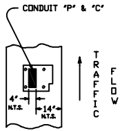
ISLAND DETAIL (ALSO SEE DWG No 99-267)
