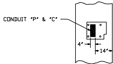
ISLAND DETAIL (ALSO SEE DWG No 99-267)
