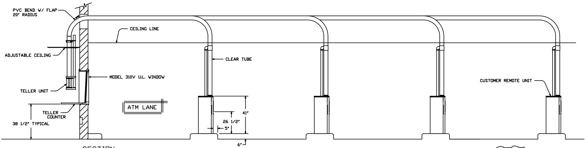
SECTION
