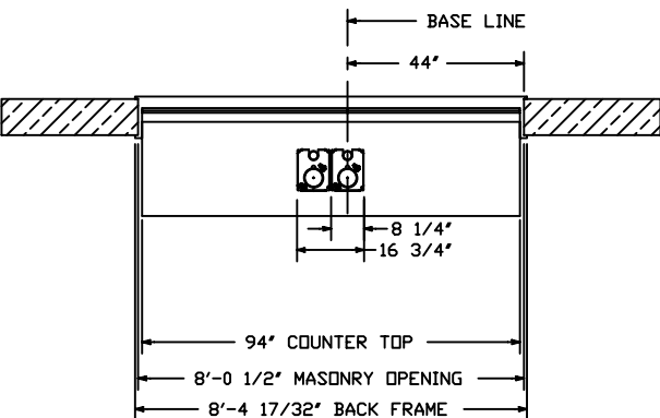
PLAN - INTERIOR
