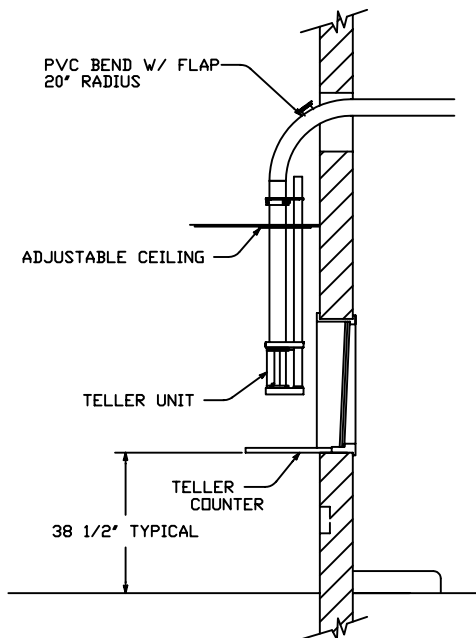
SECTION
