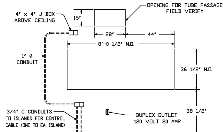
MASONRY DETAIL (FOR MODEL 038V U.L. WINDOW)
