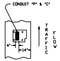
ISLAND DETAIL (ALSO SEE DWG No 99-267)
