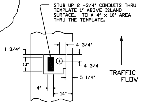
CUSTOMER UNIT TEMPLATE (ALSO SEE DWG. 99-350)
