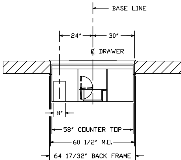
PLAN - INTERIOR
