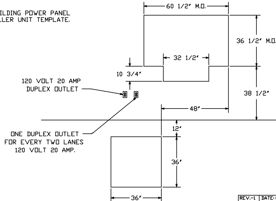
MASONRY DETAIL (FOR MODEL 035D U.L. WINDOW)
