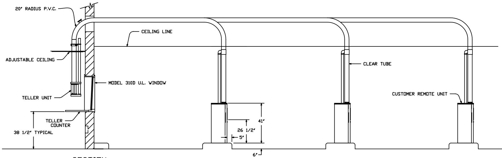
SECTION
