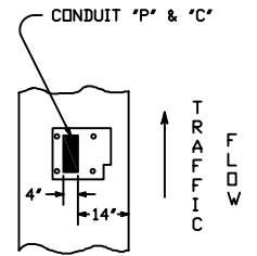
ISLAND DETAIL (ALSO SEE DWG No 99-267)
