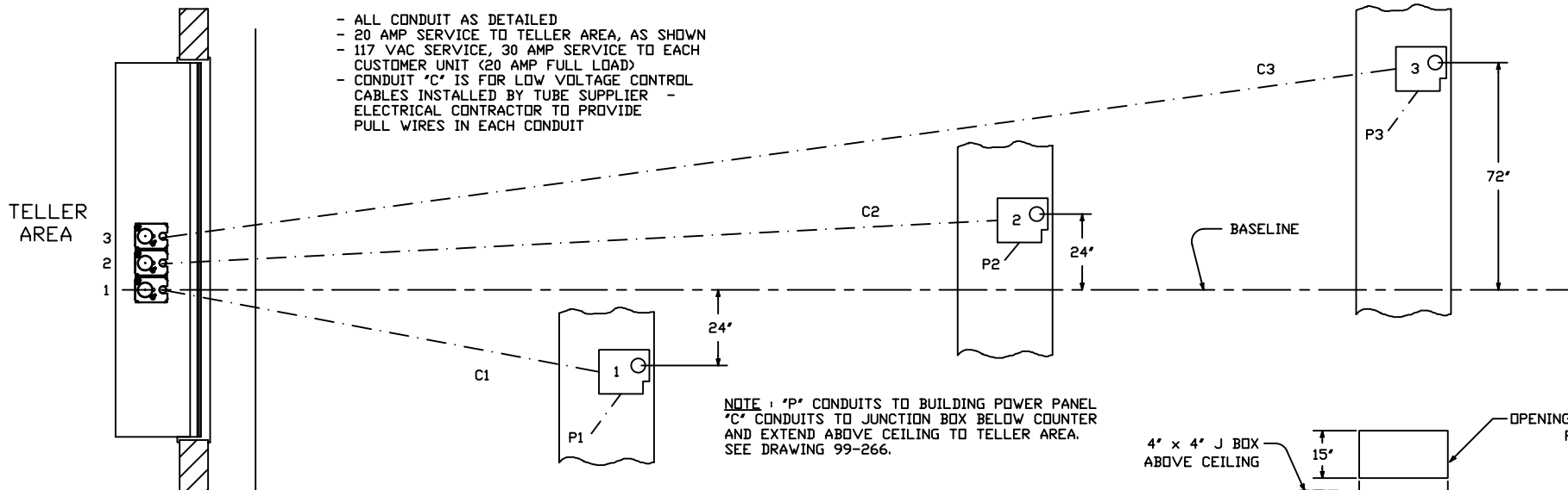
PLAN
