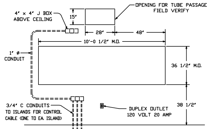
MASONRY DETAIL (FOR MODEL 310V U.L. WINDOW)
