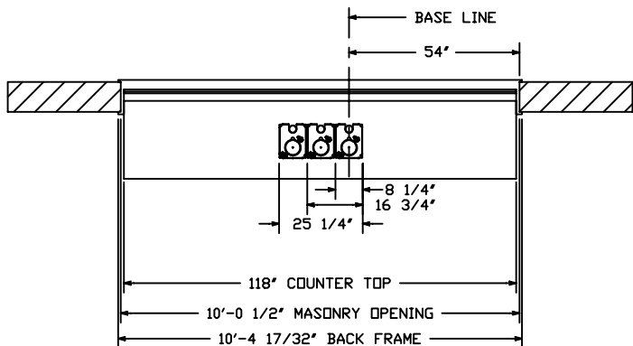
PLAN - INTERIOR
