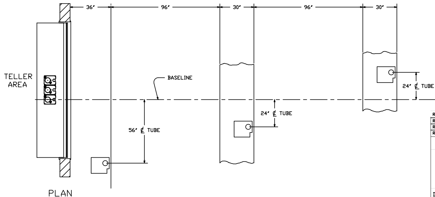
ISLAND DETAIL (ALSO SEE DWG No 99-267)
