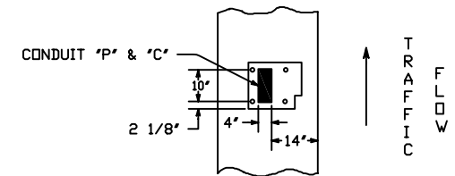
ISLAND DETAIL (ALSO SEE DWG No 99-267)
