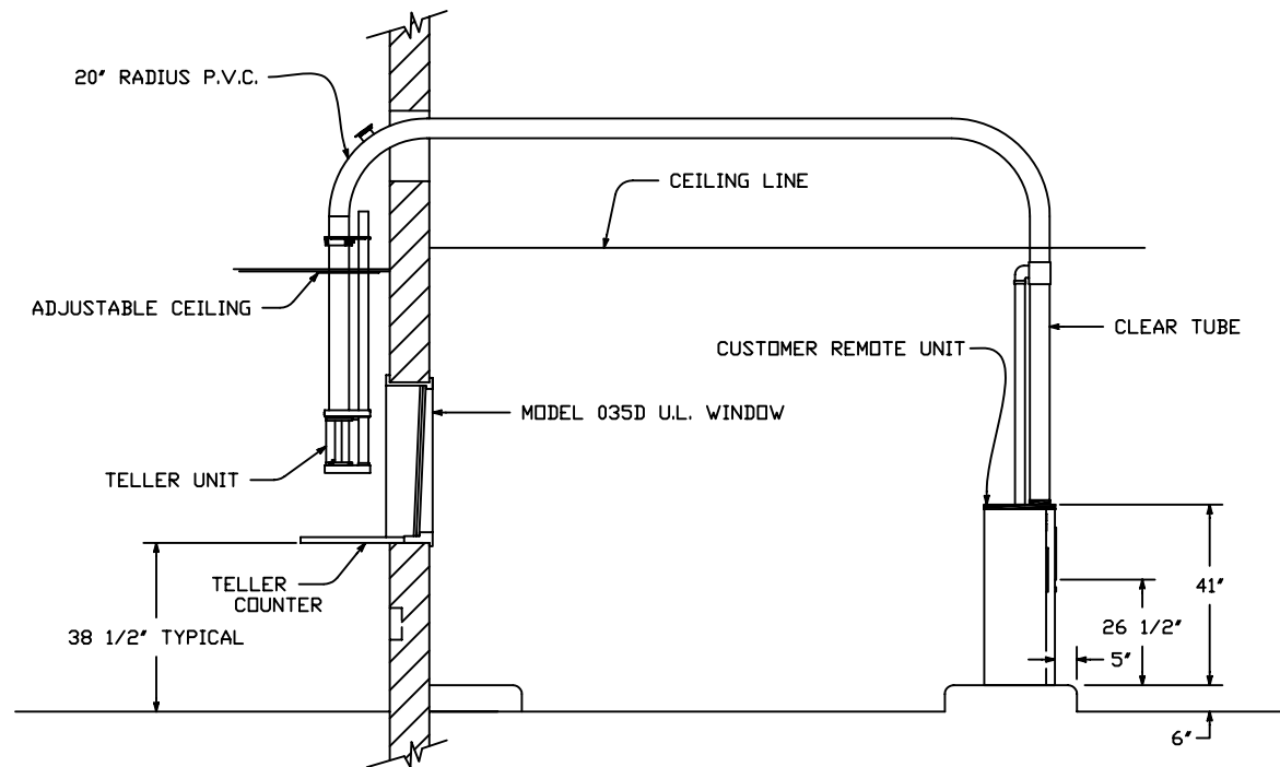
SECTION
