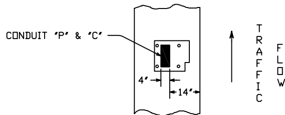
ISLAND DETAIL (ALSO SEE DWG No 99-267)
