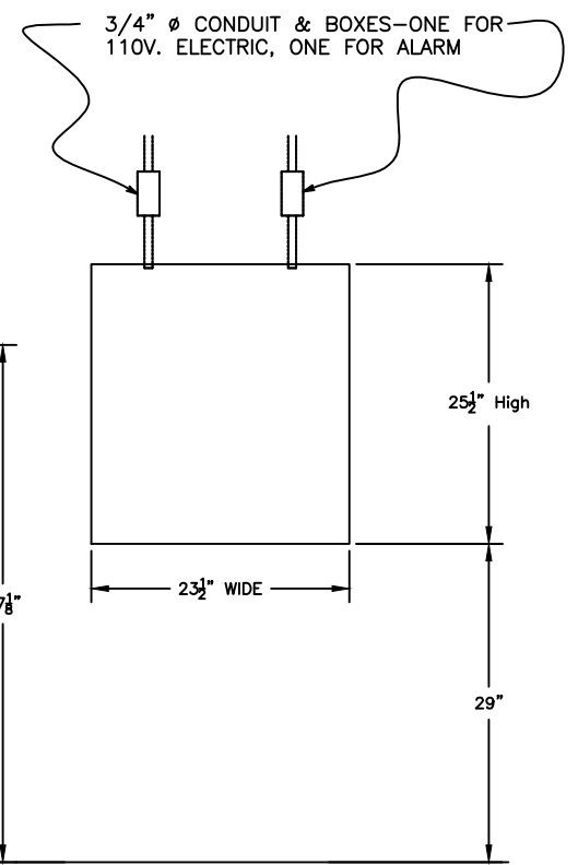
MASONRY DETAIL (VIEWED FROM OUTSIDE)
