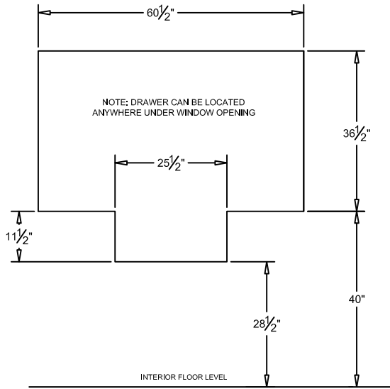
MASONRY OPENING INTERIOR
