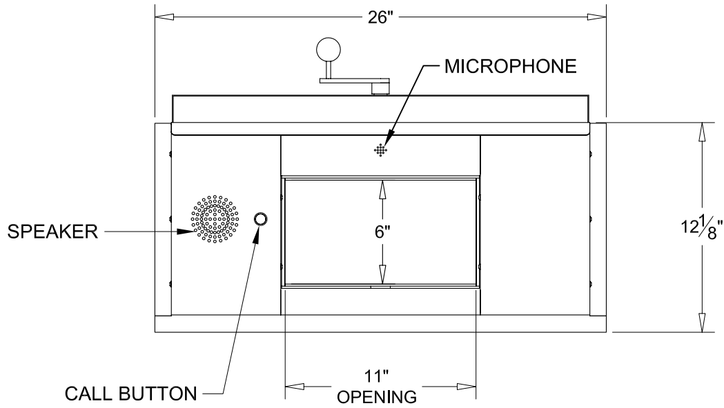
FRONT VIEW
