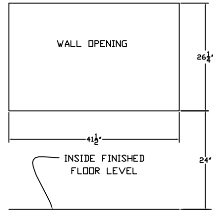
MASONRY DETAIL (AS VIEWED FROM INSIDE)
