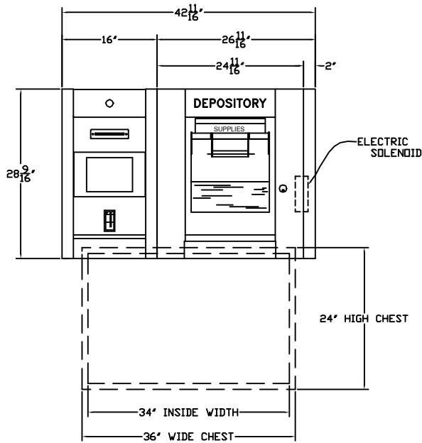
EXTERIOR ELEVATION
