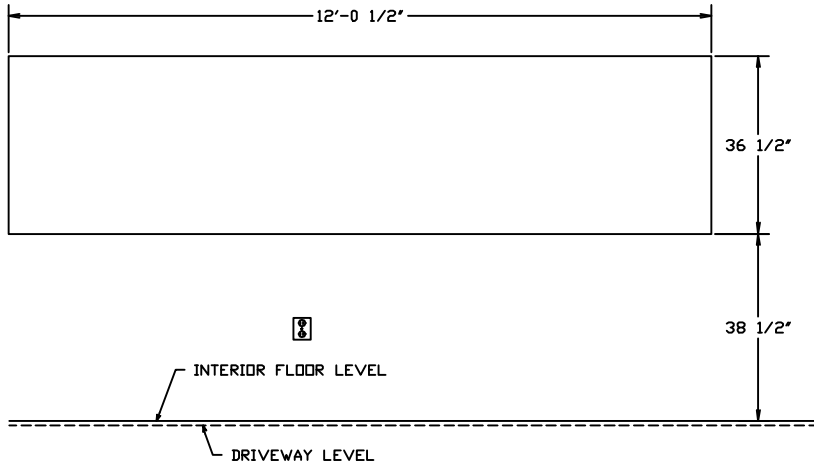
MASONRY OPENING - INTERIOR DETAIL
