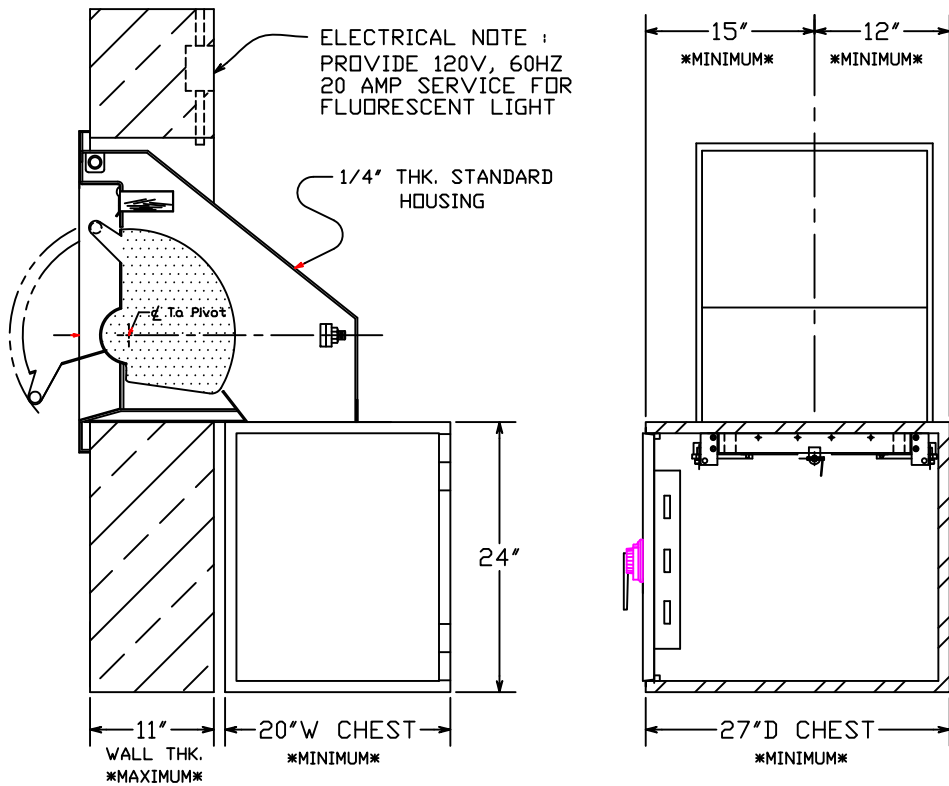
SECTION-SIDE ENTRY
