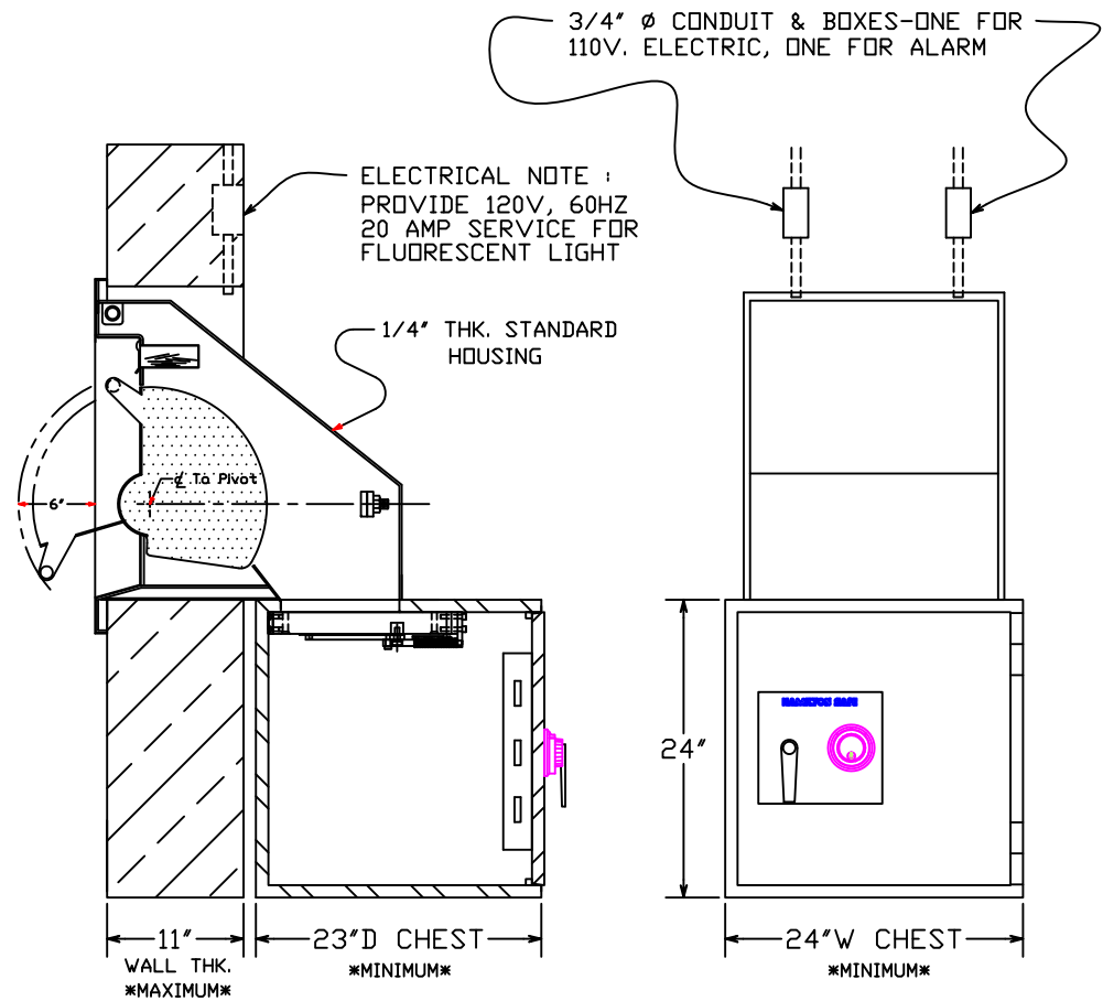
SECTION-REAR ENTRY
